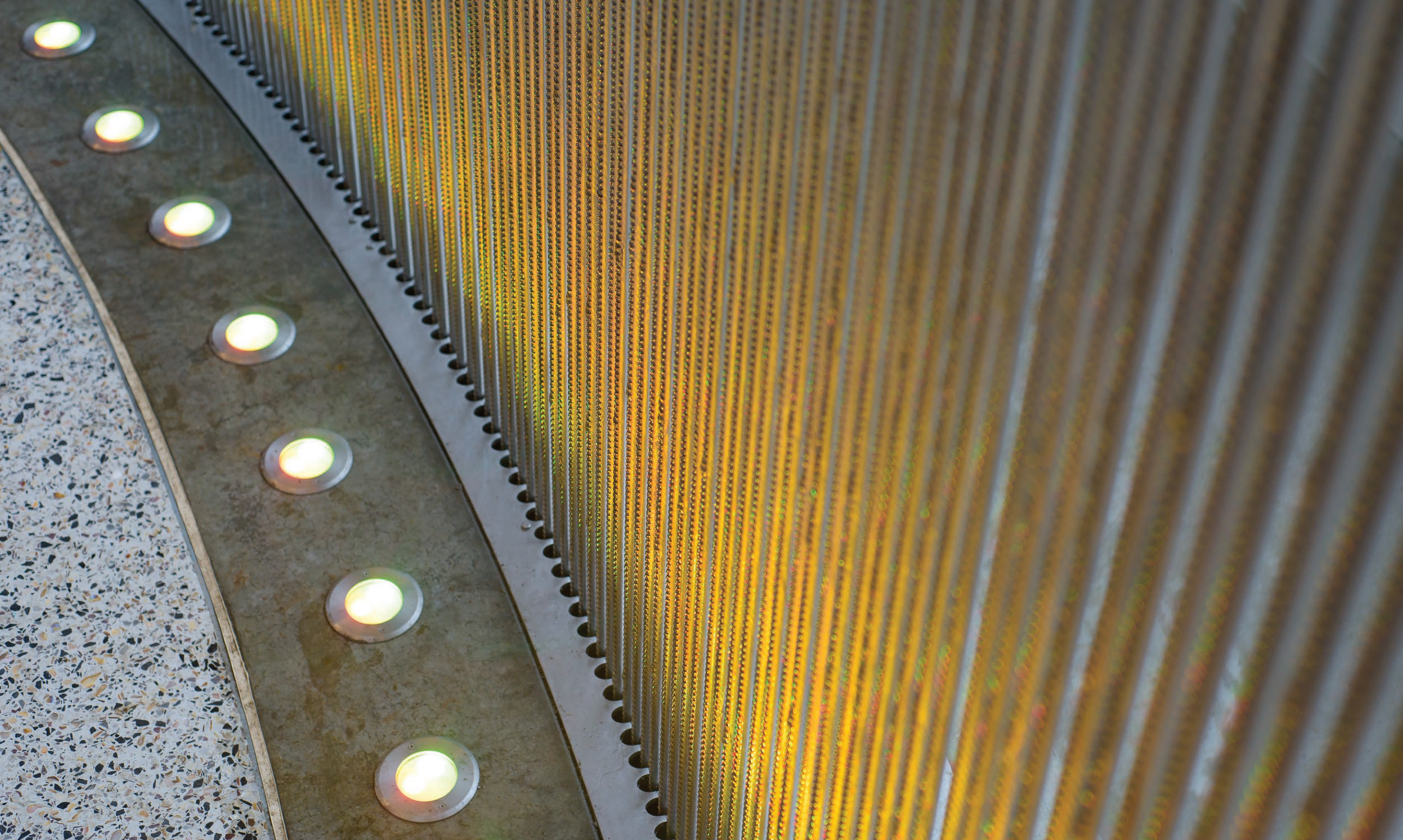
7 Park Pavilion water wall detail – Water travels down a series of thin grooved structural rods that hold the flow of water through meniscus tension, creating a dynamic water texture that appears almost as a kind of digital pixilation.
